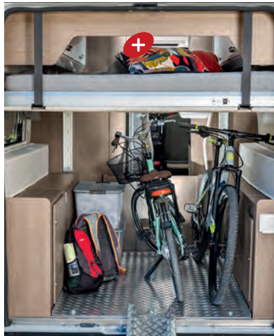
+ Daytime position : The (electric) fold-down bed lies flat against the ceiling or in its intermediate position, freeing up a large living space and/or storage space Night position: In its low position, the bed becomes extra large: 190 x 190 cm
