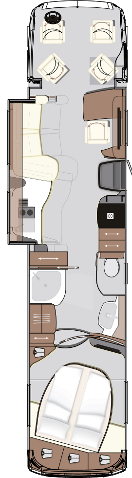
Smart 3
